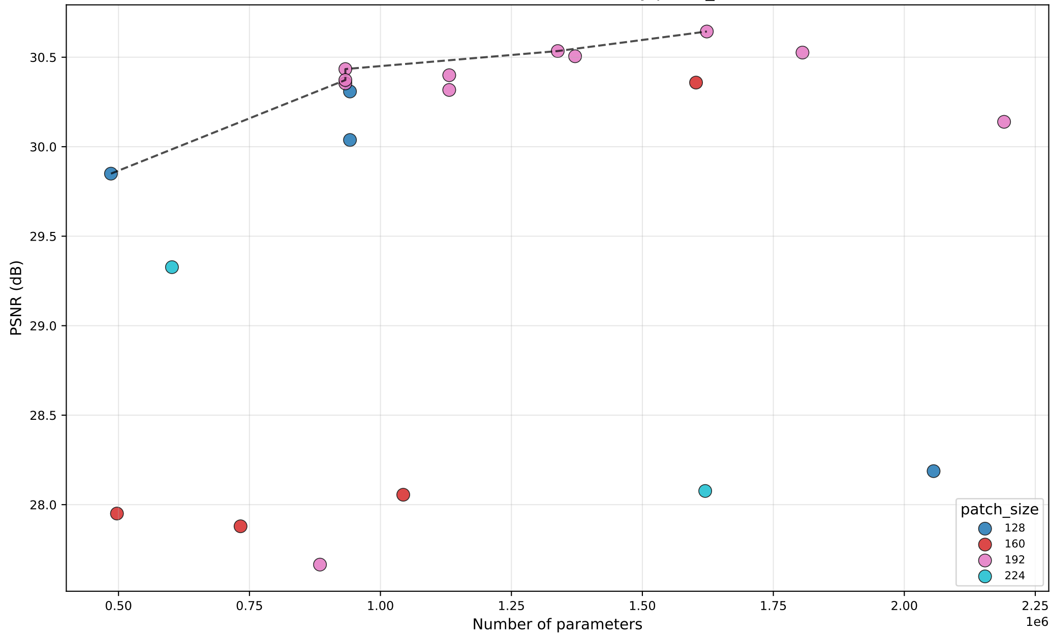
PSNR vs #Params — ELAN — by patch_size
